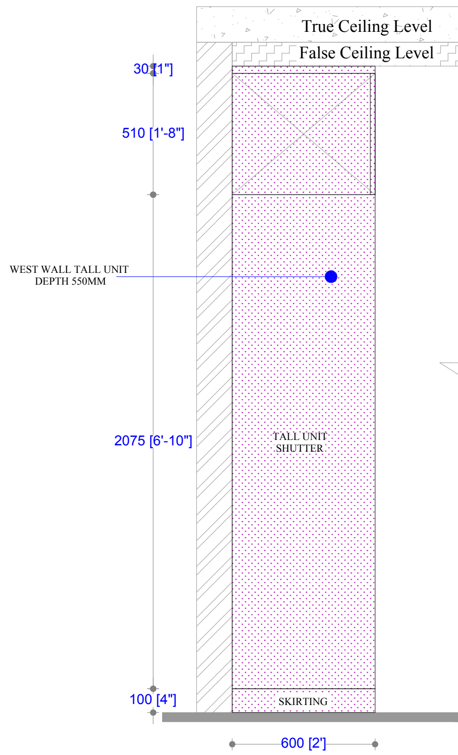
ELEVATION-C (EXTERNALS)
