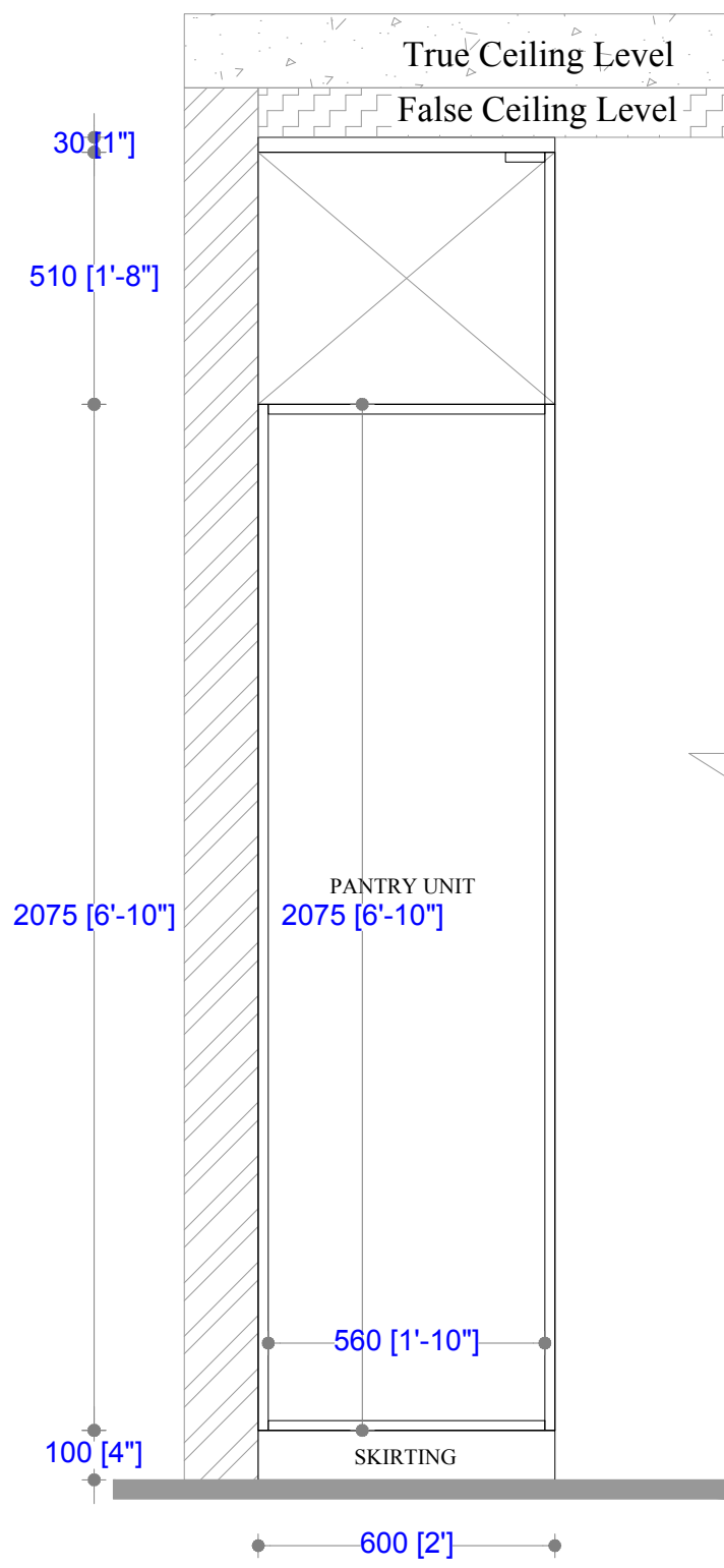
ELEVATION-C (INTERNALS)
