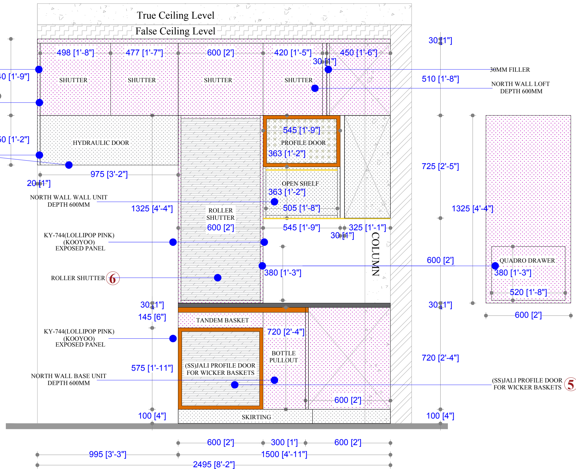
ELEVATION-D (EXTERNALS)
