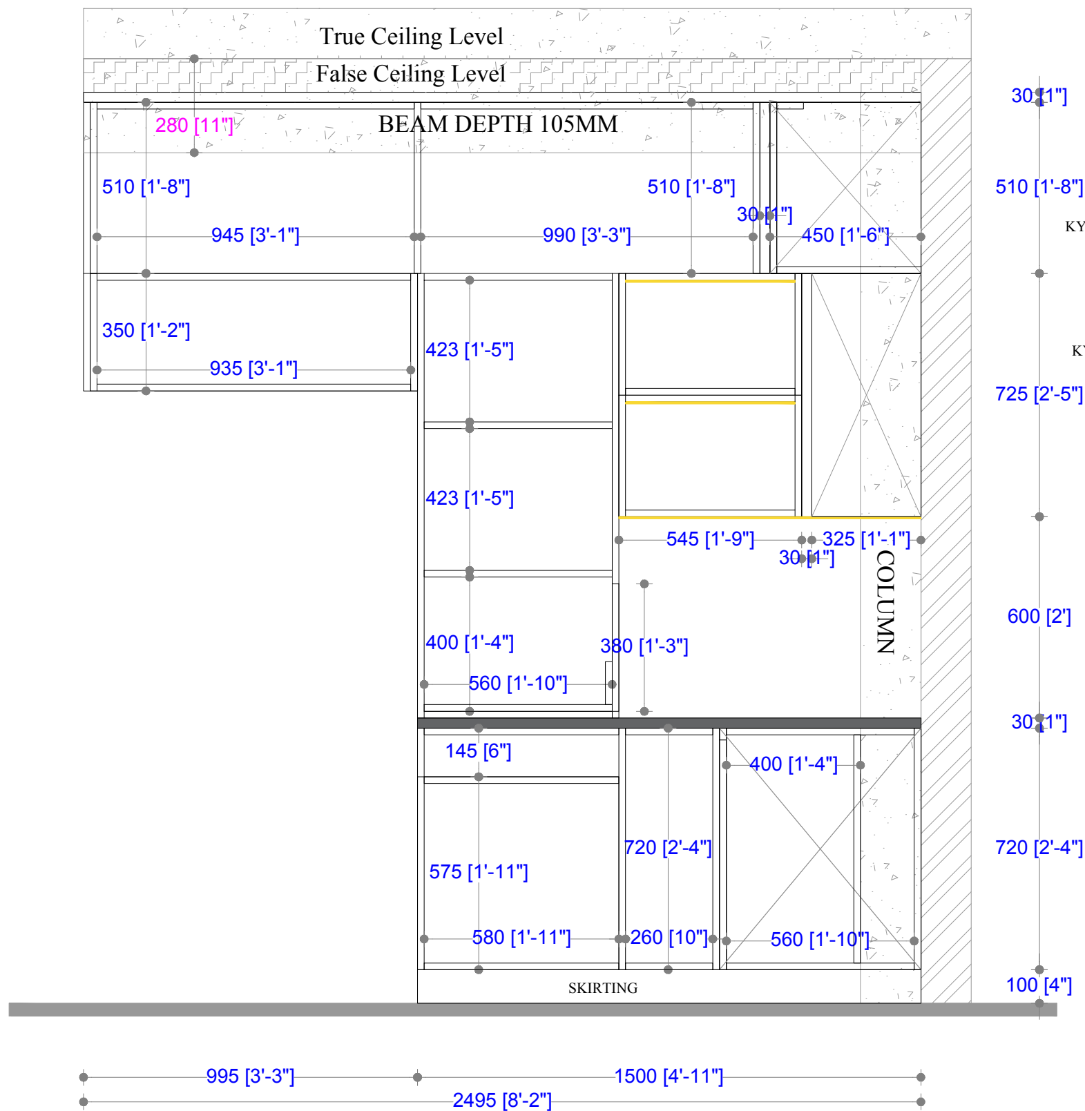
ELEVATION-D (INTERNALS)
